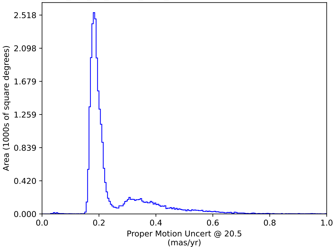
too_elab_r16_d3_ugrizy_v3.4_10yrs : Proper Motion Uncert @ 20.5
