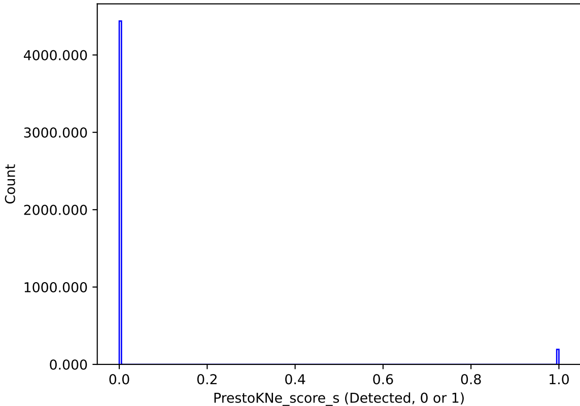
too_elab_r16_d3_ugrizy_v3.4_10yrs : PrestoKNe_score_s
