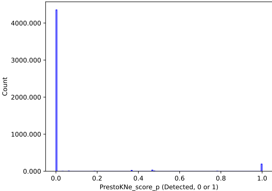
too_elab_r16_d3_ugrizy_v3.4_10yrs : PrestoKNe_score_p
