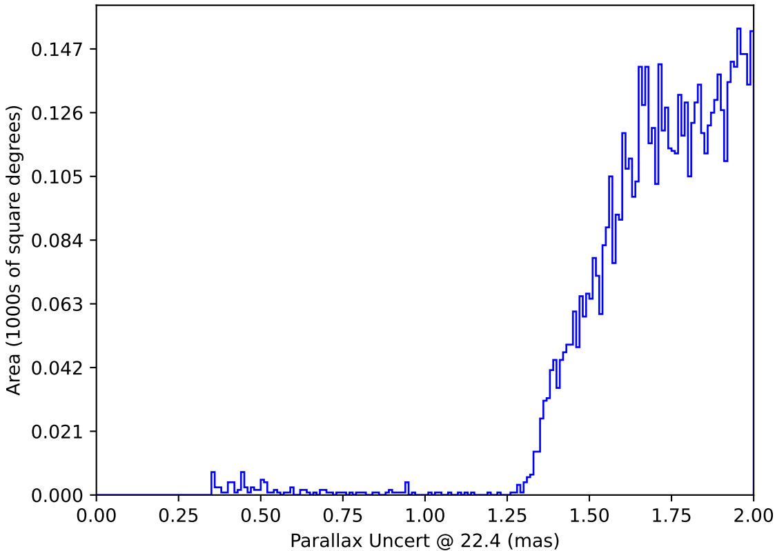
too_elab_r16_d3_ugrizy_v3.4_10yrs : Parallax Uncert @ 22.4
