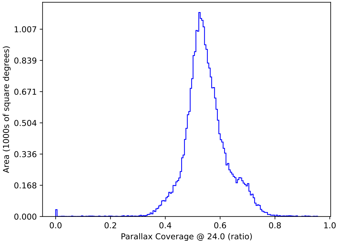
too_elab_r16_d3_ugrizy_v3.4_10yrs : Parallax Coverage @ 24.0
