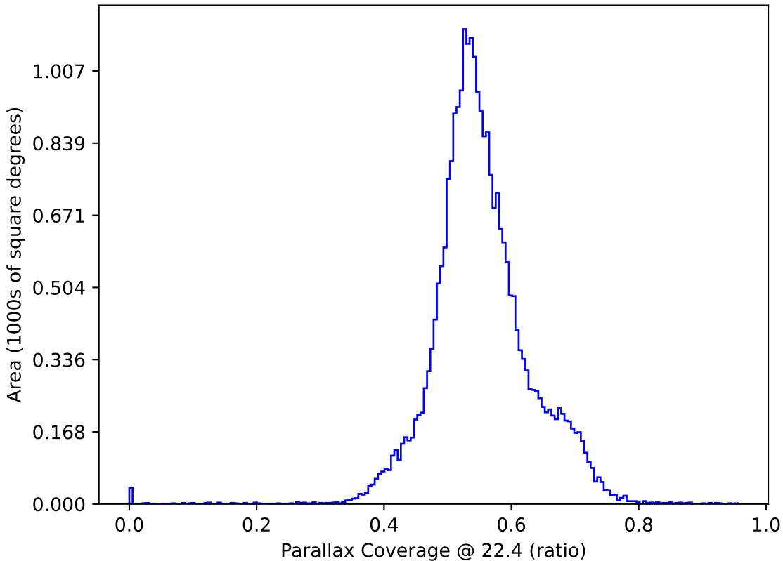
too_elab_r16_d3_ugrizy_v3.4_10yrs : Parallax Coverage @ 22.4
