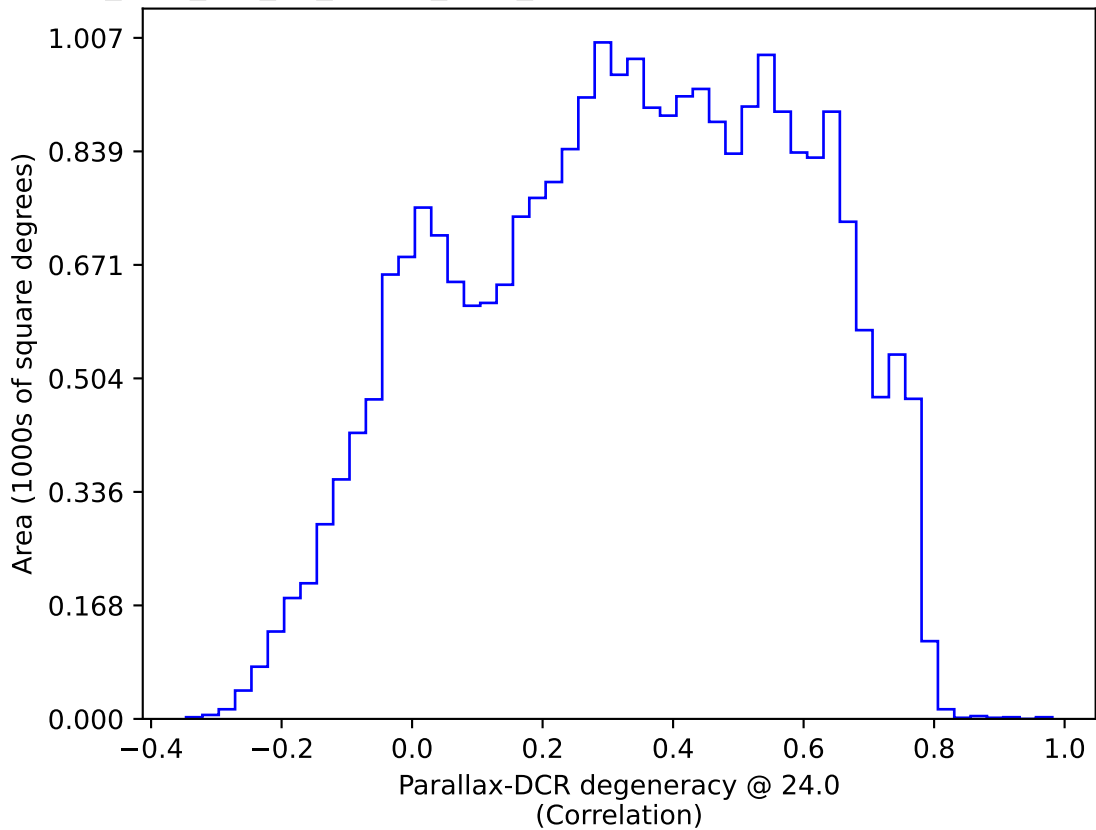
too_elab_r16_d3_ugrizy_v3.4_10yrs : Parallax-DCR degeneracy @ 24.0
