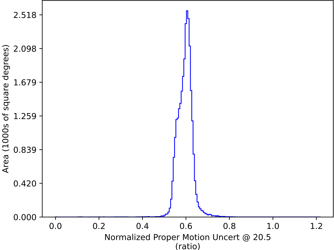
too_elab_r16_d3_ugrizy_v3.4_10yrs : Normalized Proper Motion Uncert @ 20.5
