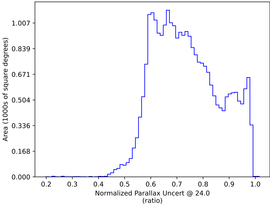
too_elab_r16_d3_ugrizy_v3.4_10yrs : Normalized Parallax Uncert @ 24.0
