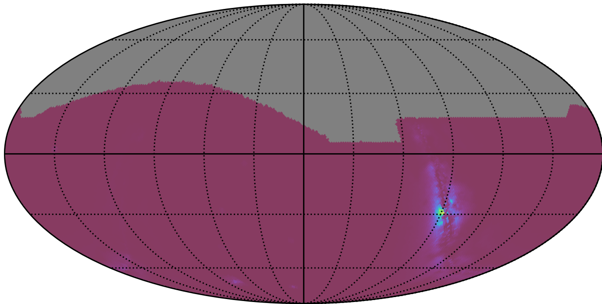
too_elab_r16_d3_ugrizy_v3.4_10yrs : NlcPoints
