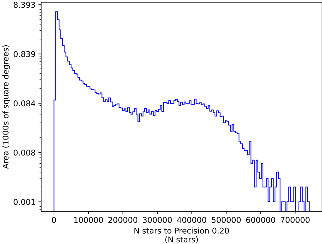
too_elab_r16_d3_ugrizy_v3.4_10yrs z: N stars to Precision 0.20
