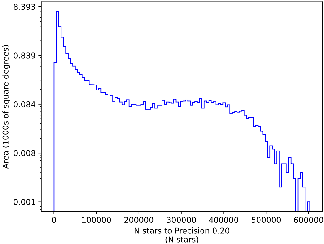
too_elab_r16_d3_ugrizy_v3.4_10yrs y: N stars to Precision 0.20
