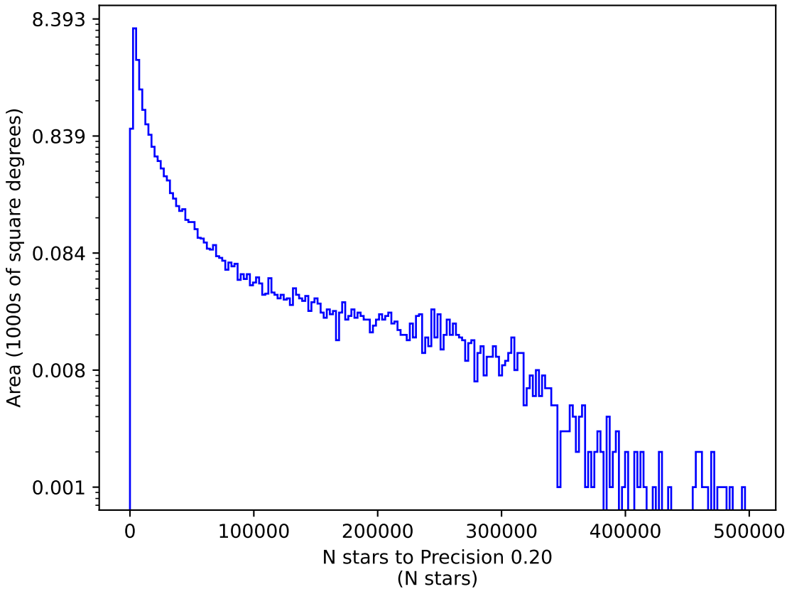
too_elab_r16_d3_ugrizy_v3.4_10yrs u: N stars to Precision 0.20
