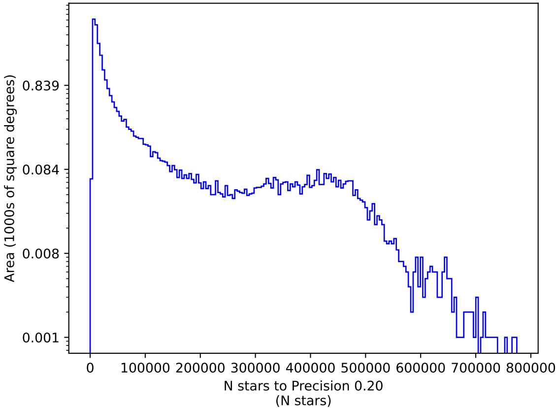
too_elab_r16_d3_ugrizy_v3.4_10yrs r: N stars to Precision 0.20
