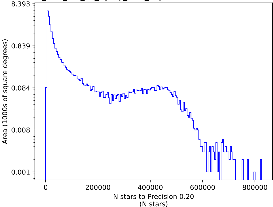
too_elab_r16_d3_ugrizy_v3.4_10yrs i: N stars to Precision 0.20
