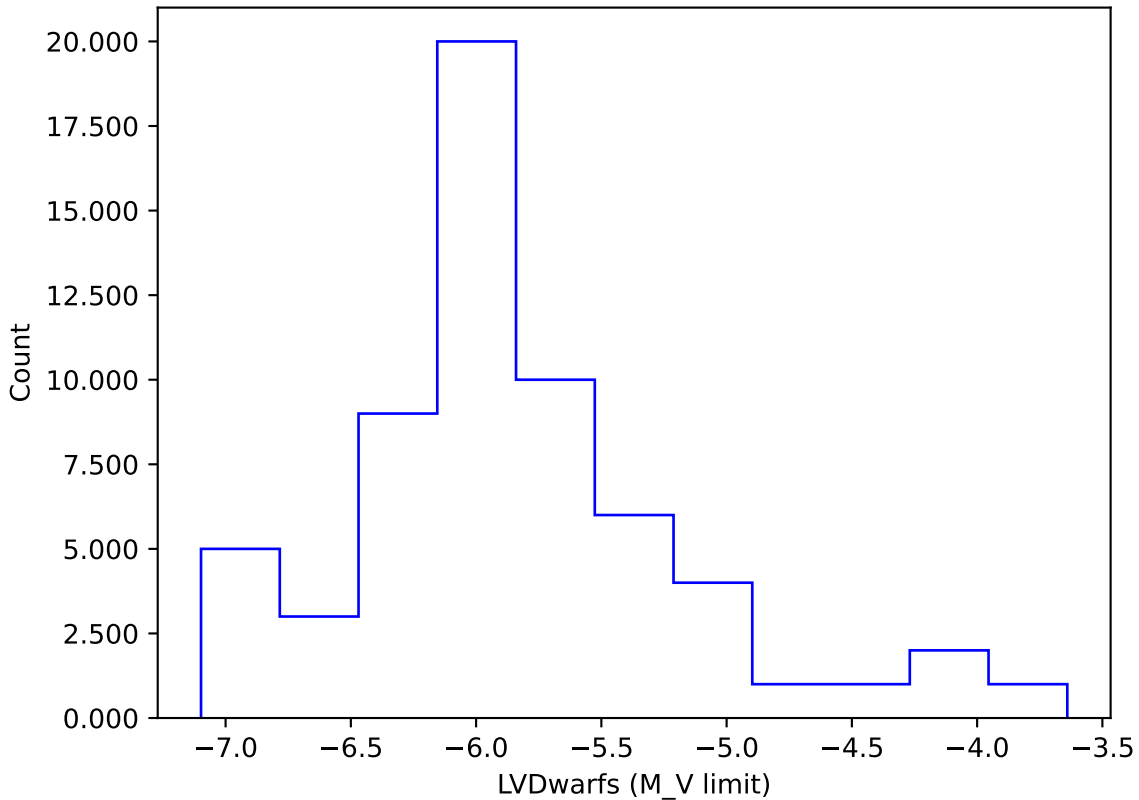
too_elab_r16_d3_ugrizy_v3.4_10yrs gi: LVDwarfs
