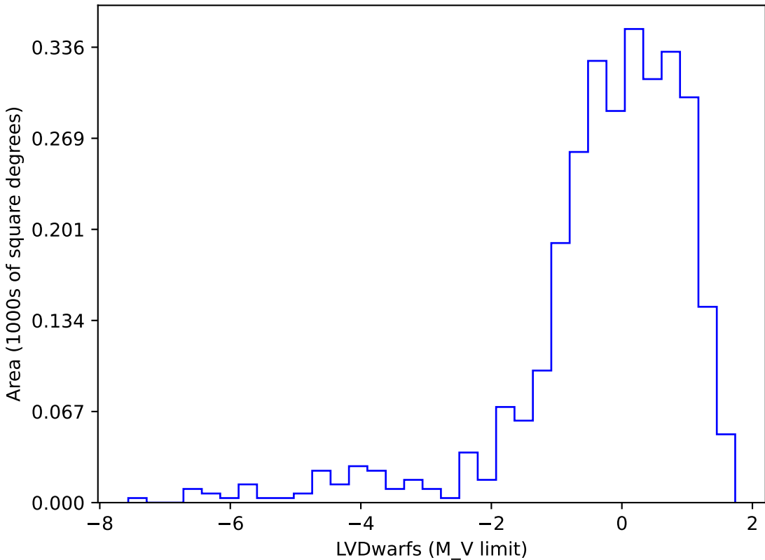
too_elab_r16_d3_ugrizy_v3.4_10yrs gi SCP: LVDwarfs
