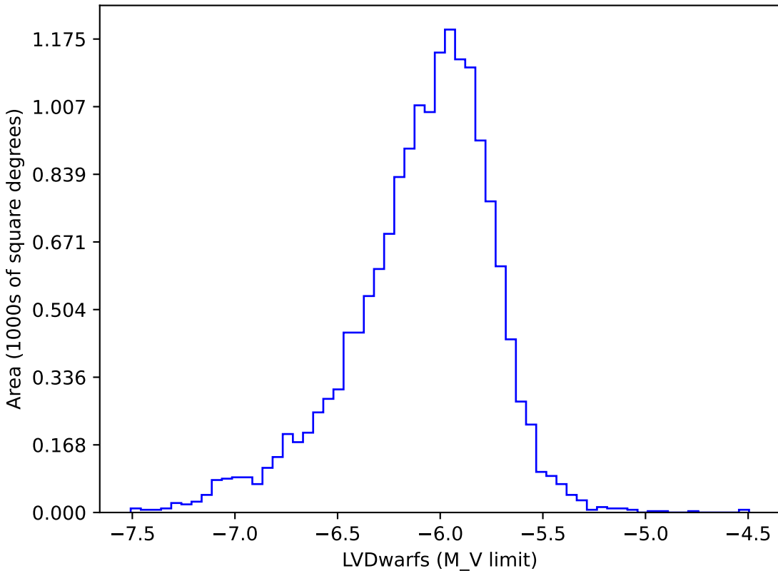
too_elab_r16_d3_ugrizy_v3.4_10yrs gi: LVDwarfs
