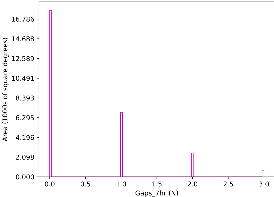
too_elab_r16_d3_ugrizy_v3.4_10yrs z band: Gaps_7hr
