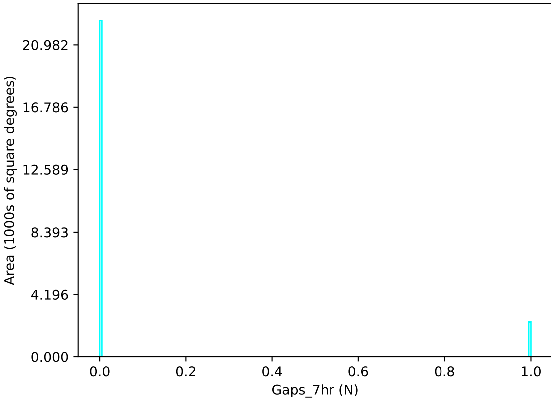
too_elab_r16_d3_ugrizy_v3.4_10yrs u band: Gaps_7hr
