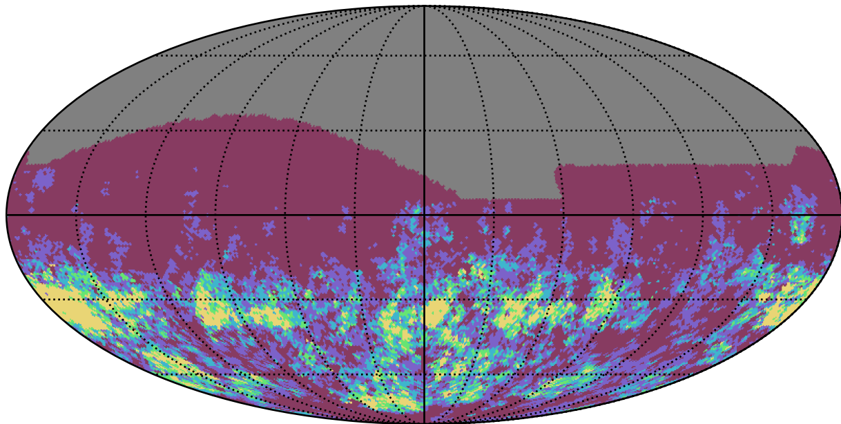
too_elab_r16_d3_ugrizy_v3.4_10yrs r band: Gaps_7hr
