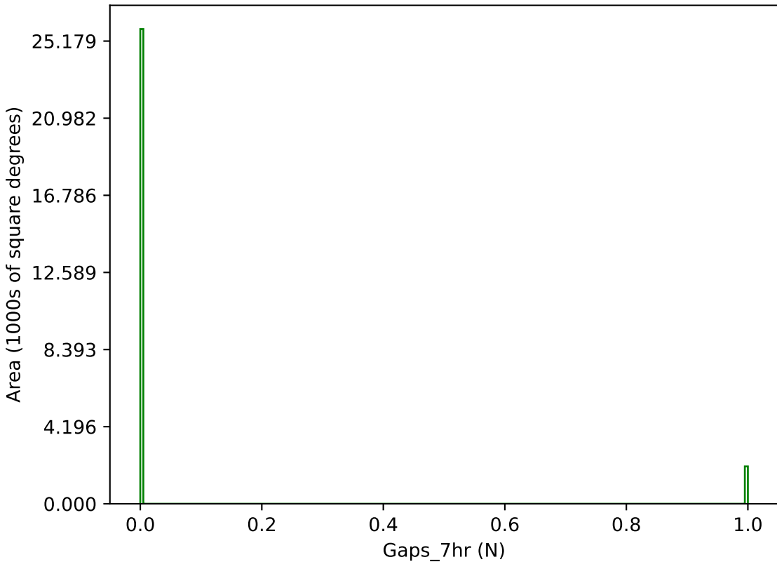
too_elab_r16_d3_ugrizy_v3.4_10yrs g band: Gaps_7hr
