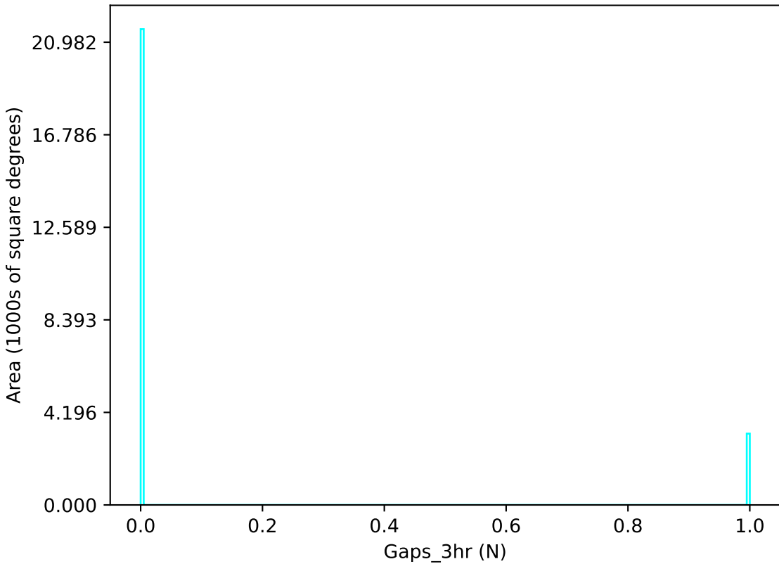
too_elab_r16_d3_ugrizy_v3.4_10yrs u band: Gaps_3hr
