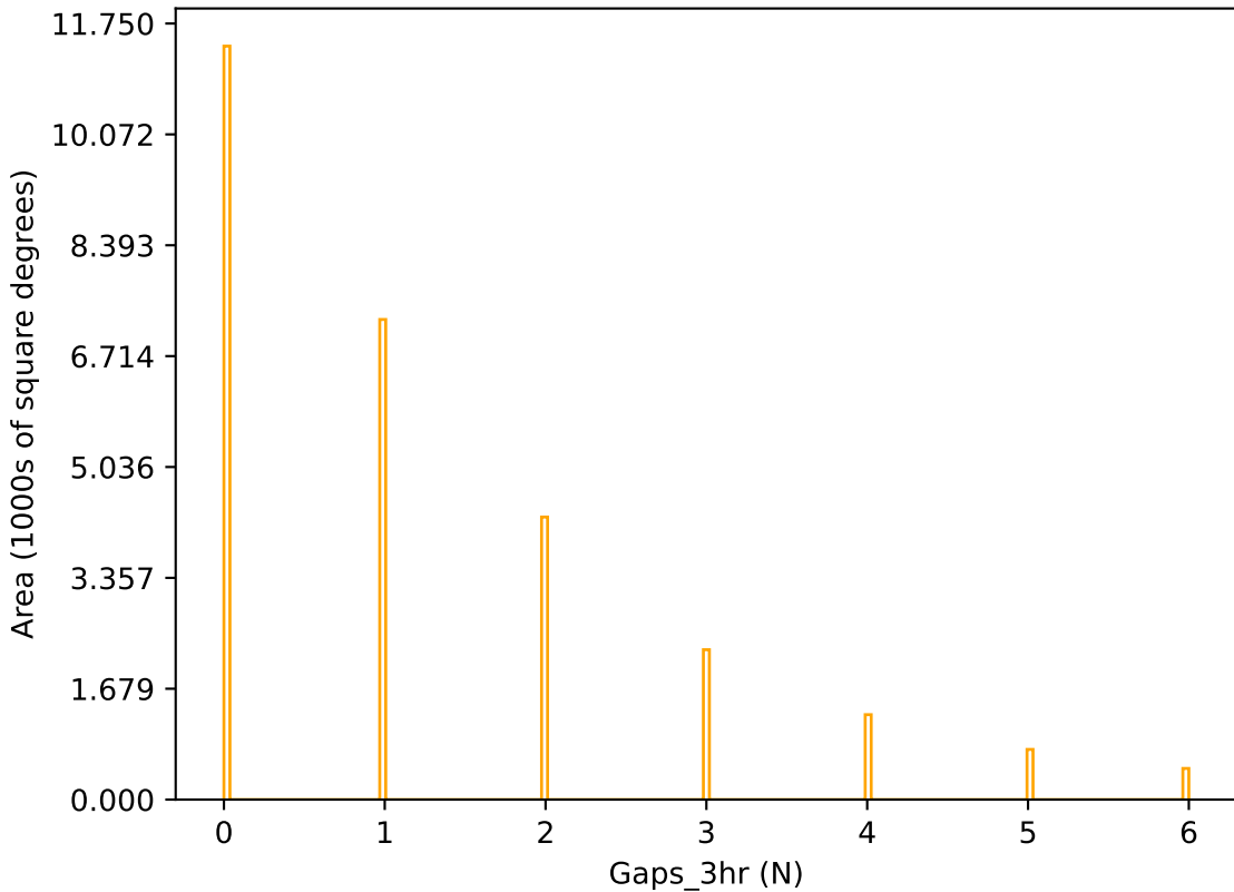
too_elab_r16_d3_ugrizy_v3.4_10yrs r band: Gaps_3hr
