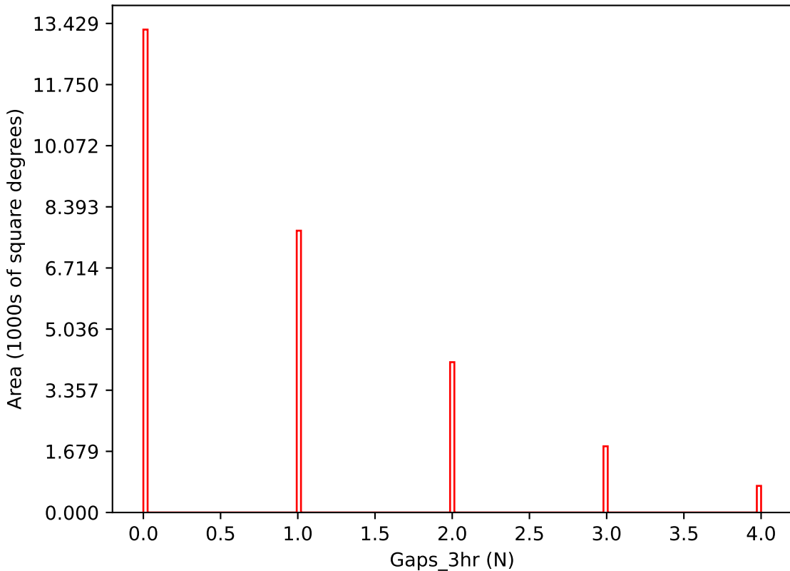
too_elab_r16_d3_ugrizy_v3.4_10yrs i band: Gaps_3hr
