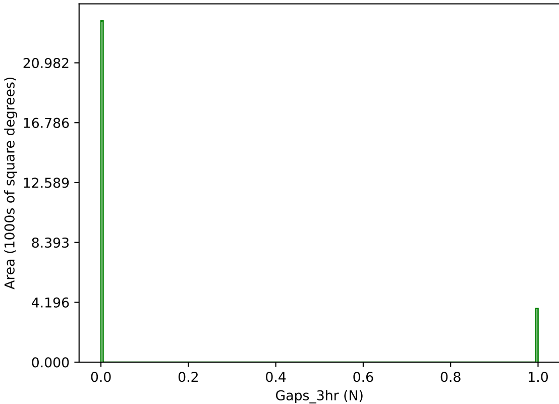
too_elab_r16_d3_ugrizy_v3.4_10yrs g band: Gaps_3hr
