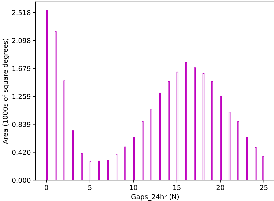
too_elab_r16_d3_ugrizy_v3.4_10yrs z band: Gaps_24hr
