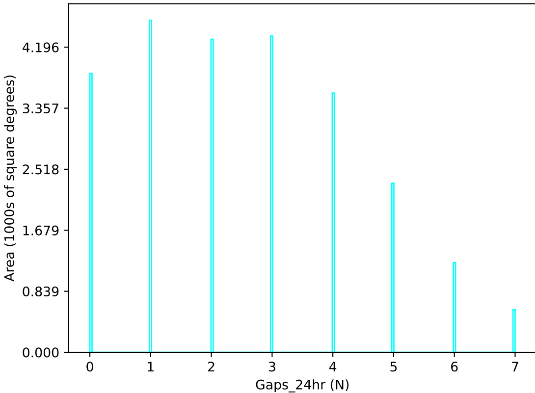
too_elab_r16_d3_ugrizy_v3.4_10yrs u band: Gaps_24hr
