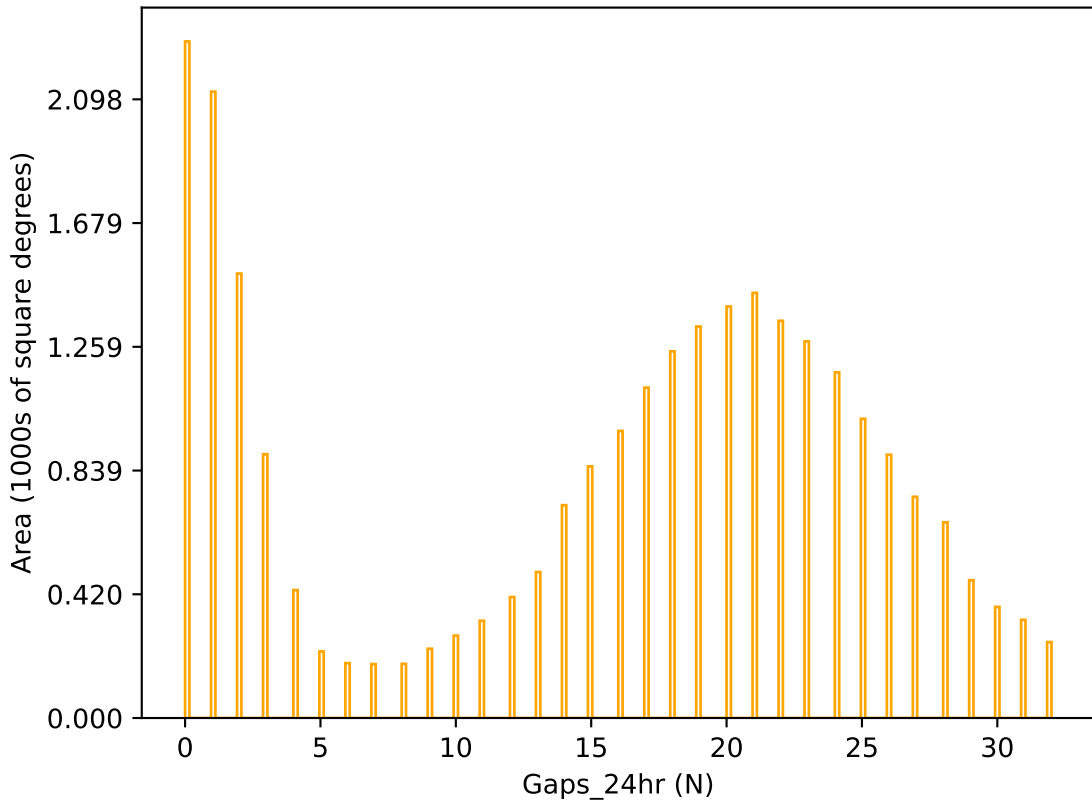
too_elab_r16_d3_ugrizy_v3.4_10yrs r band: Gaps_24hr
