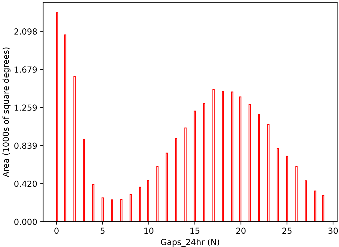
too_elab_r16_d3_ugrizy_v3.4_10yrs i band: Gaps_24hr
