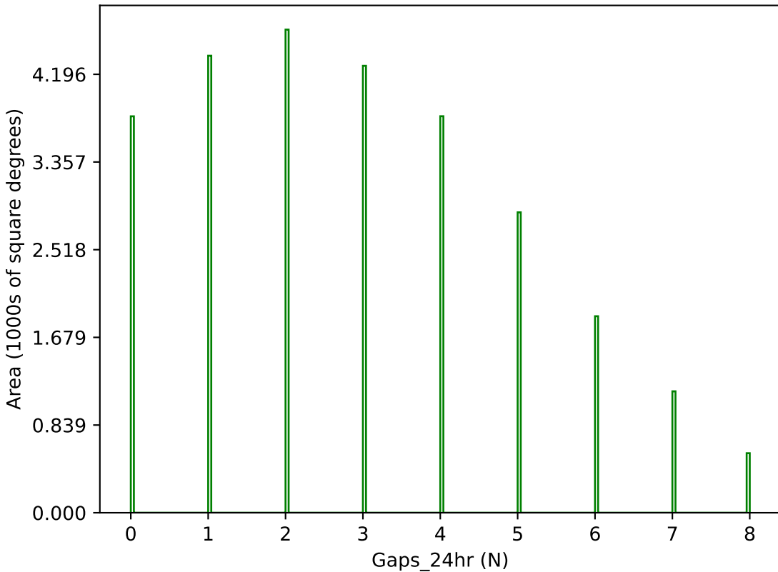
too_elab_r16_d3_ugrizy_v3.4_10yrs g band: Gaps_24hr
