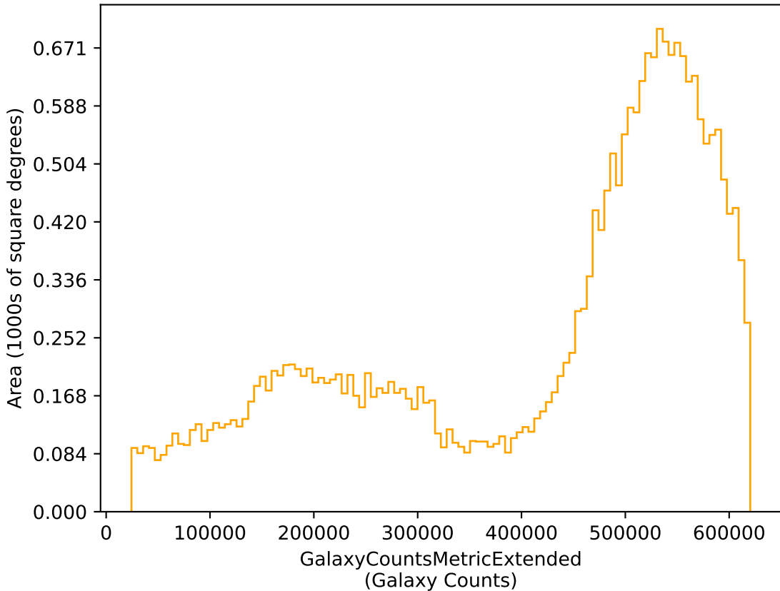
too_elab_r16_d3_ugrizy_v3.4_10yrs r: GalaxyCountsMetricExtended
