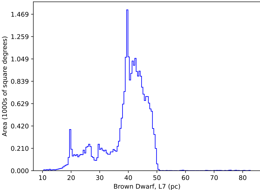
too_elab_r16_d3_ugrizy_v3.4_10yrs : Brown Dwarf, L7
