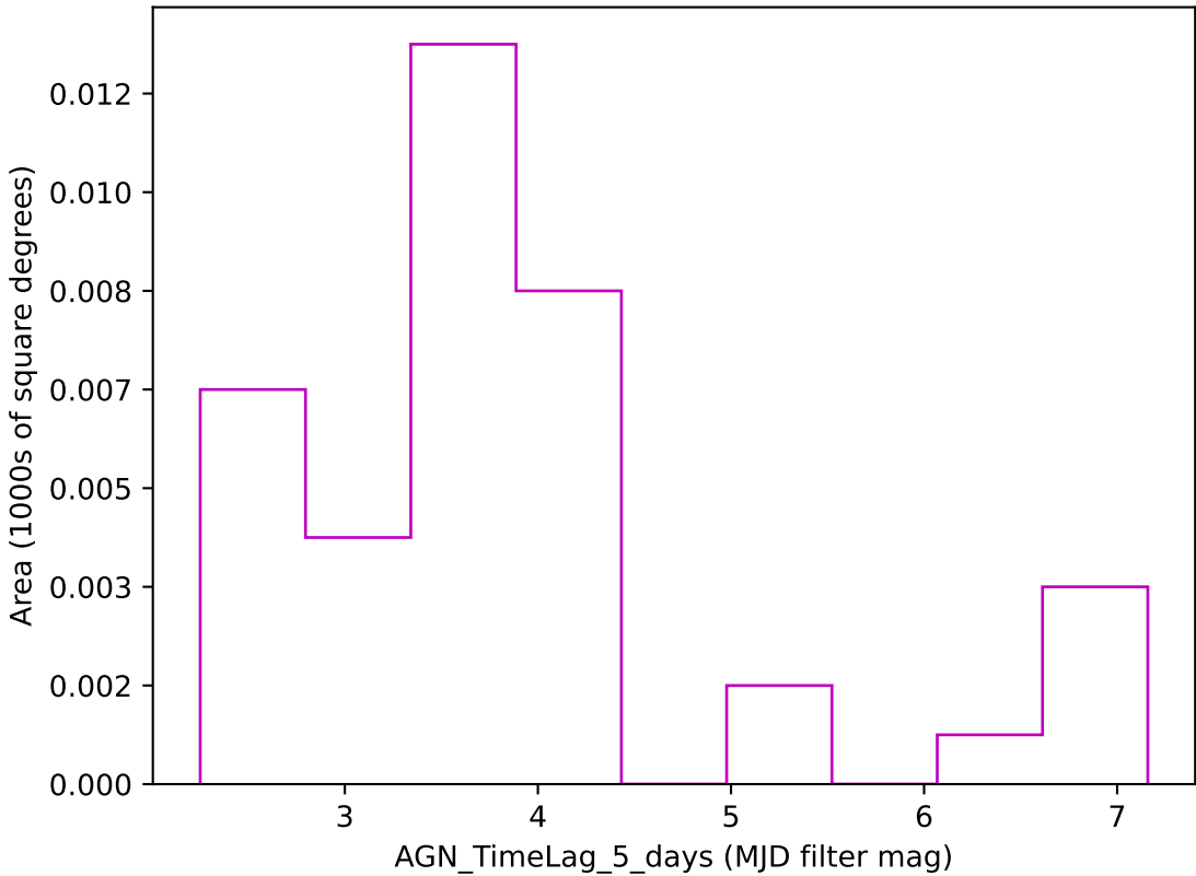
too_elab_r16_d3_ugrizy_v3.4_10yrs z band: AGN_TimeLag_5_days
