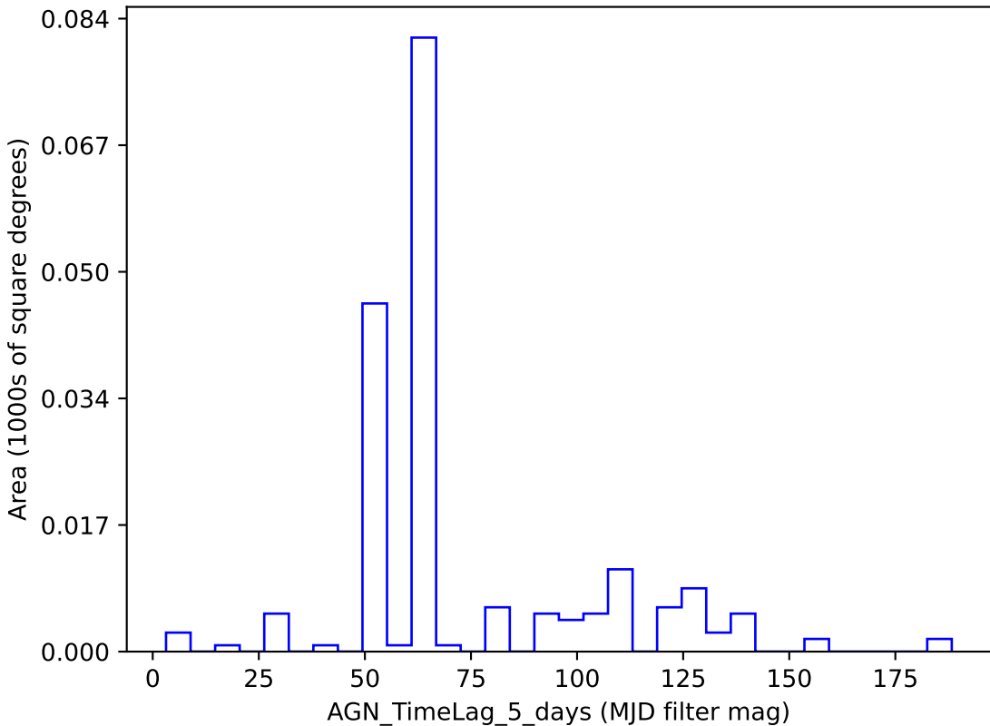
too_elab_r16_d3_ugrizy_v3.4_10yrs y band: AGN_TimeLag_5_days
