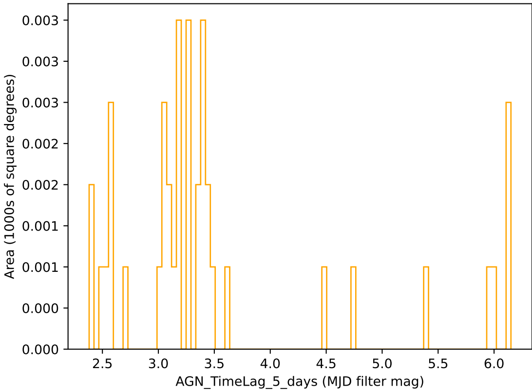
too_elab_r16_d3_ugrizy_v3.4_10yrs r band: AGN_TimeLag_5_days
