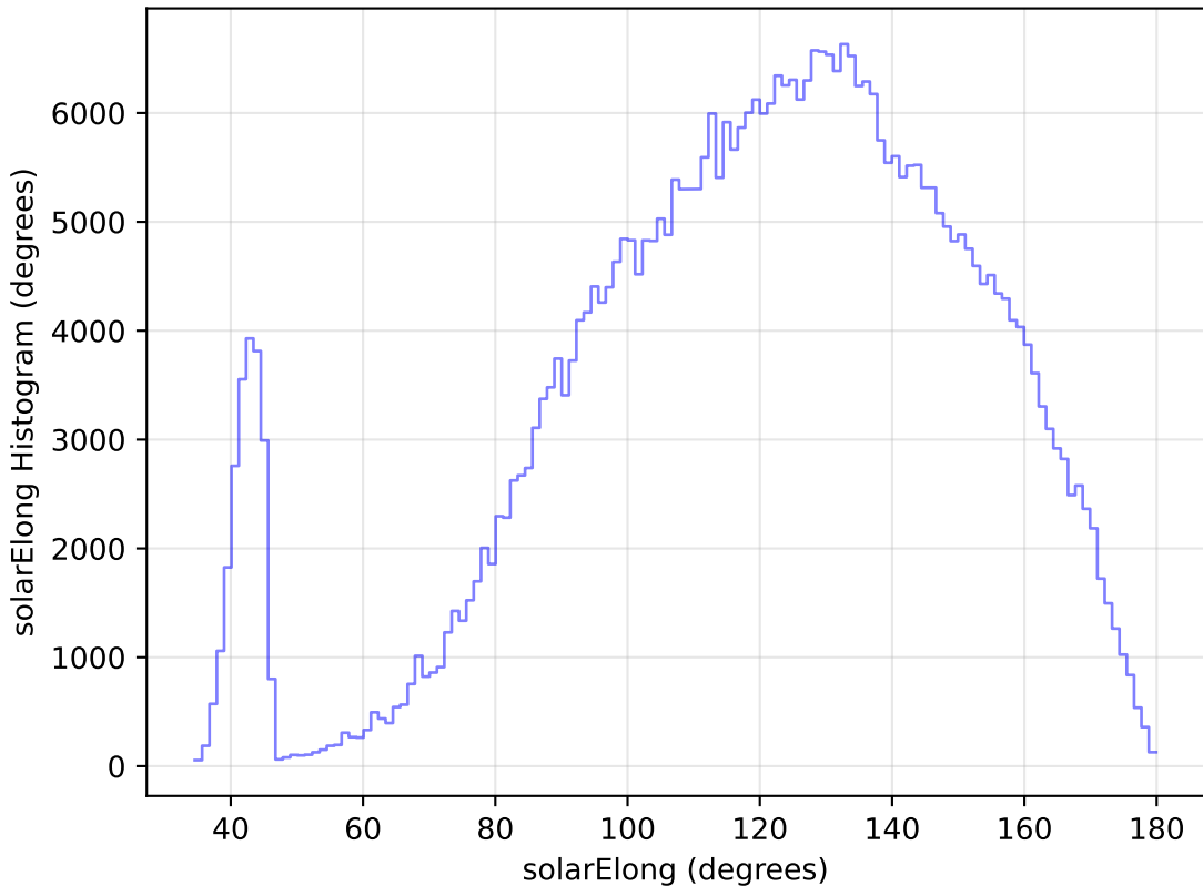
too_elab_r16_d3_ugrizy_v3.4_10yrs WFD z band: solarElong Histogram
