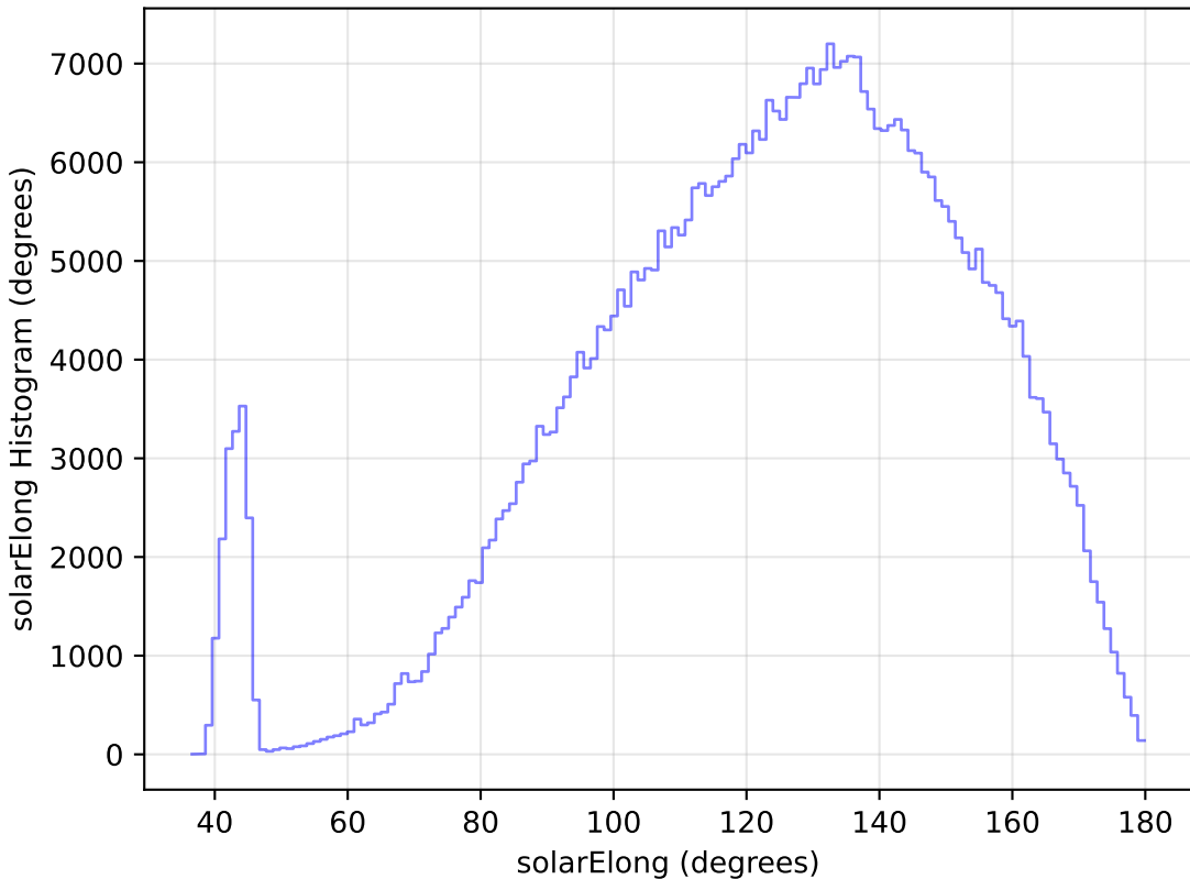
too_elab_r16_d3_ugrizy_v3.4_10yrs WFD r band: solarElong Histogram
