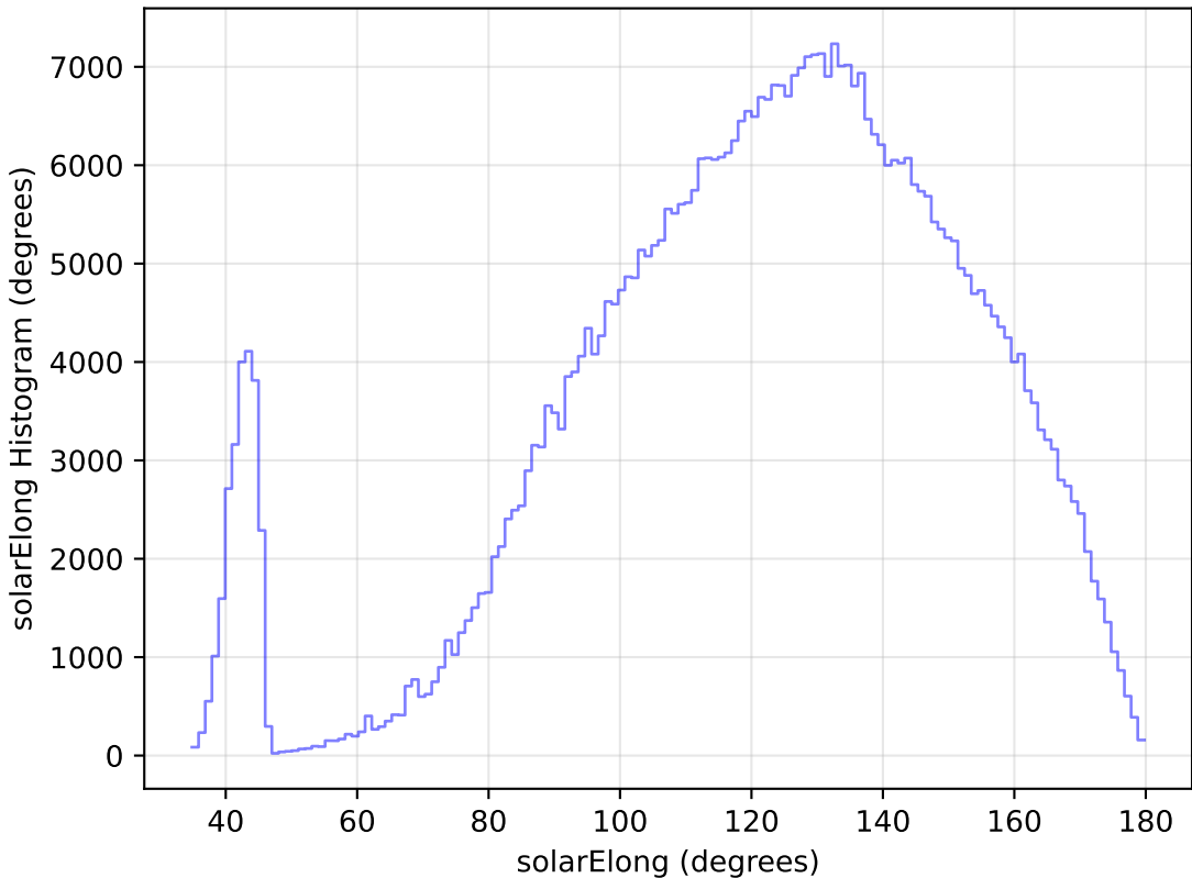
too_elab_r16_d3_ugrizy_v3.4_10yrs WFD i band: solarElong Histogram
