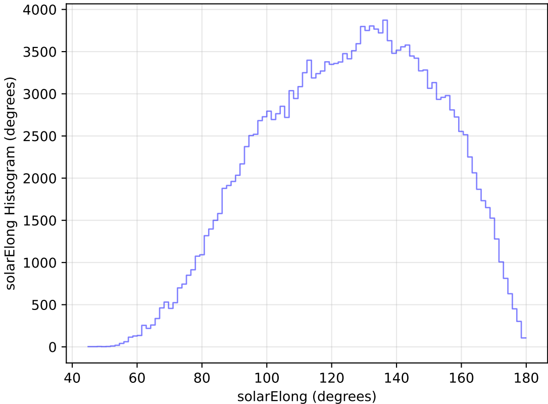
too_elab_r16_d3_ugrizy_v3.4_10yrs WFD g band: solarElong Histogram
