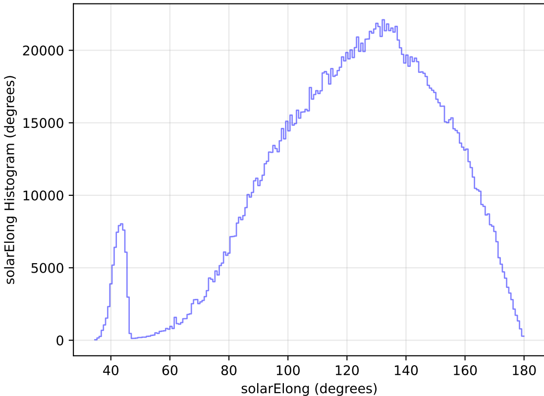
too_elab_r16_d3_ugrizy_v3.4_10yrs WFD all bands: solarElong Histogram
