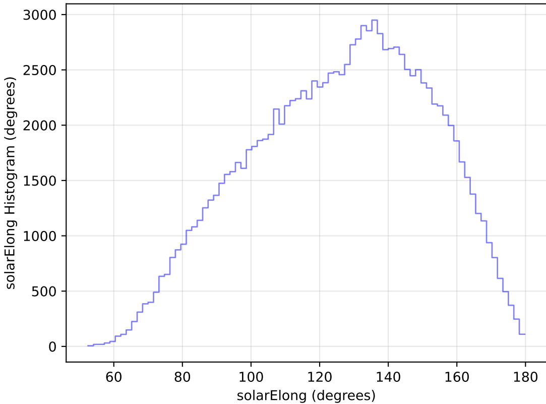
too_elab_r16_d3_ugrizy_v3.4_10yrs All sky u band: solarElong Histogram
