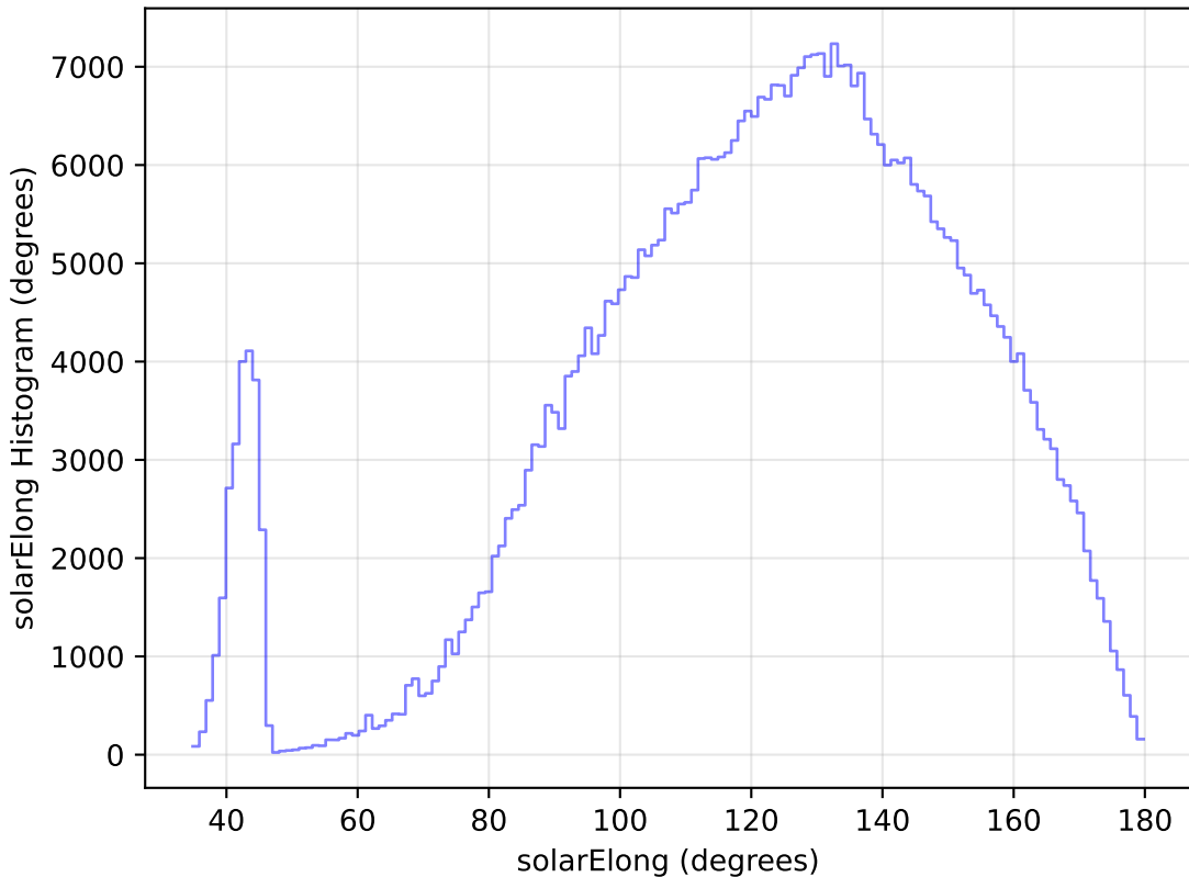
too_elab_r16_d3_ugrizy_v3.4_10yrs All sky i band: solarElong Histogram
