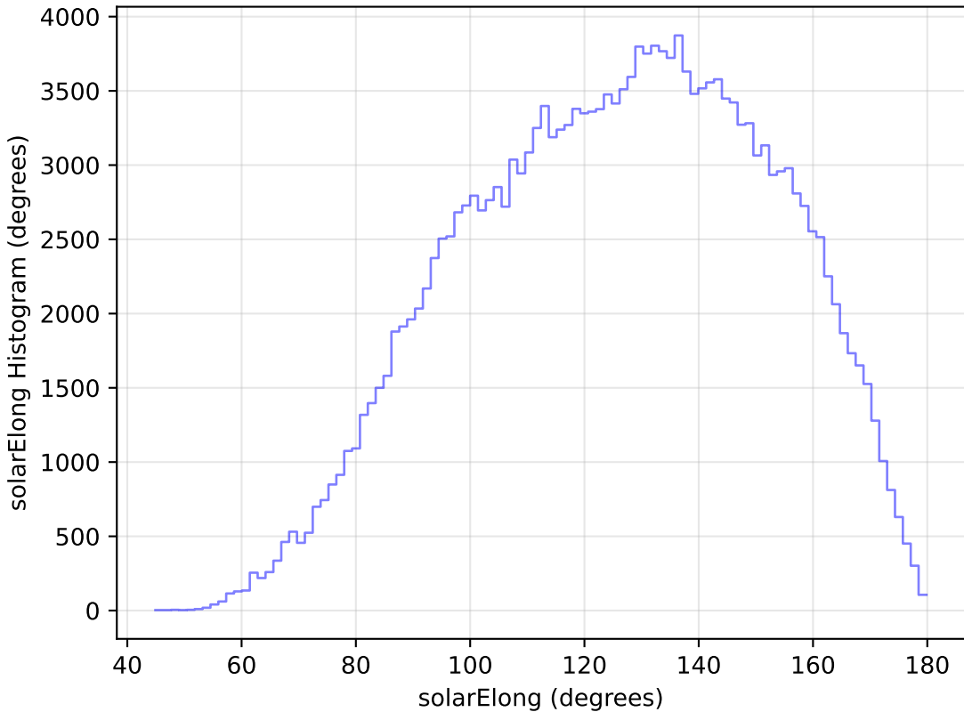
too_elab_r16_d3_ugrizy_v3.4_10yrs All sky g band: solarElong Histogram
