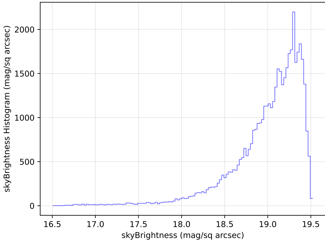
too_elab_r16_d3_ugrizy_v3.4_10yrs Yr 1 z band: skyBrightness Histogram
