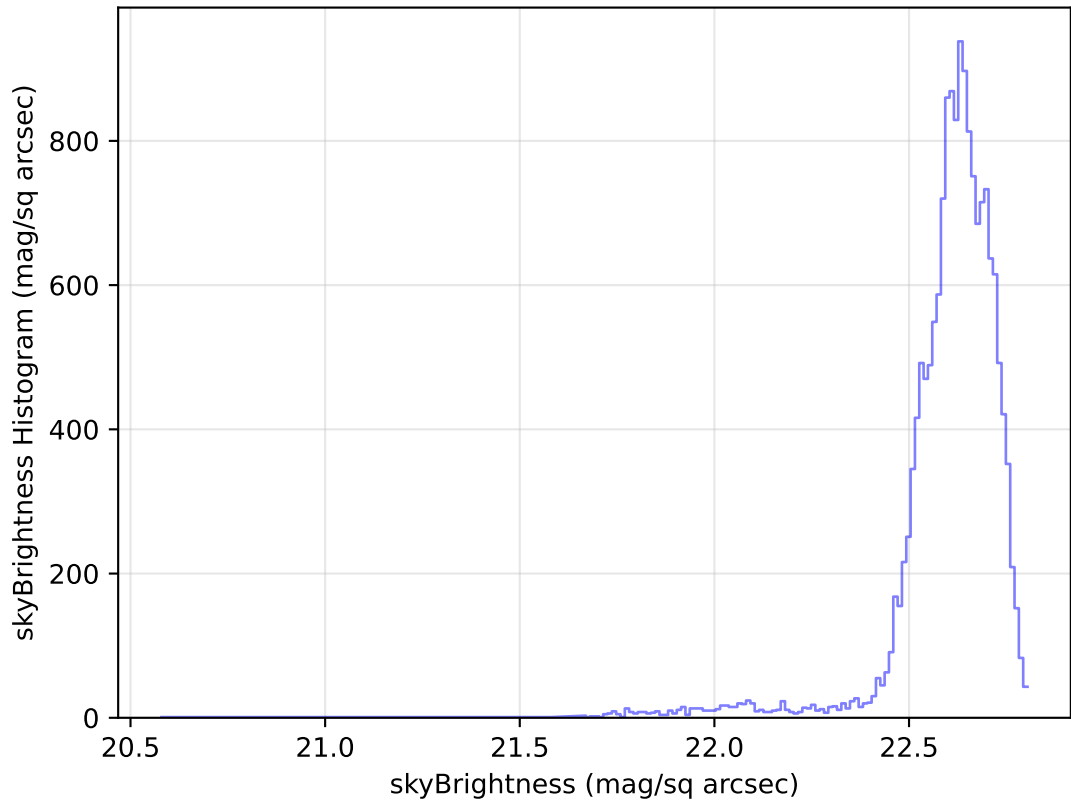
too_elab_r16_d3_ugrizy_v3.4_10yrs Yr 1 u band: skyBrightness Histogram
