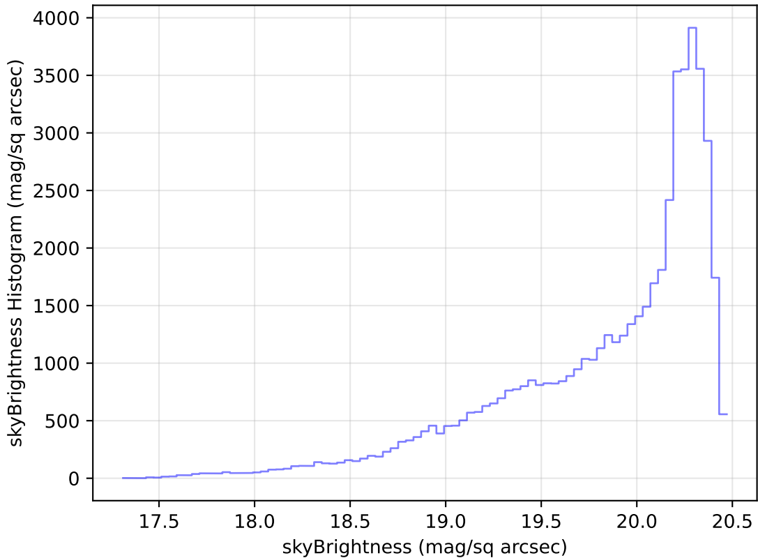
too_elab_r16_d3_ugrizy_v3.4_10yrs Yr 1 i band: skyBrightness Histogram
