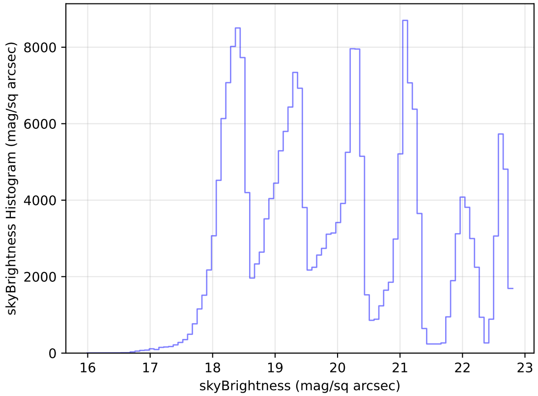
too_elab_r16_d3_ugrizy_v3.4_10yrs Yr 1 all bands: skyBrightness Histogram
