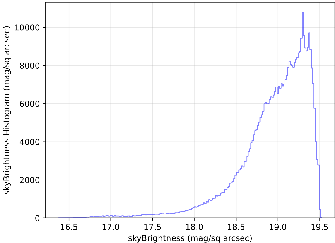
too_elab_r16_d3_ugrizy_v3.4_10yrs WFD z band: skyBrightness Histogram
