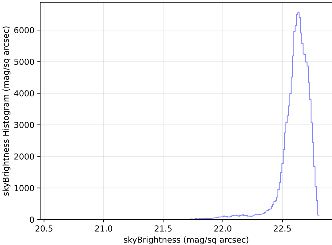
too_elab_r16_d3_ugrizy_v3.4_10yrs WFD u band: skyBrightness Histogram
